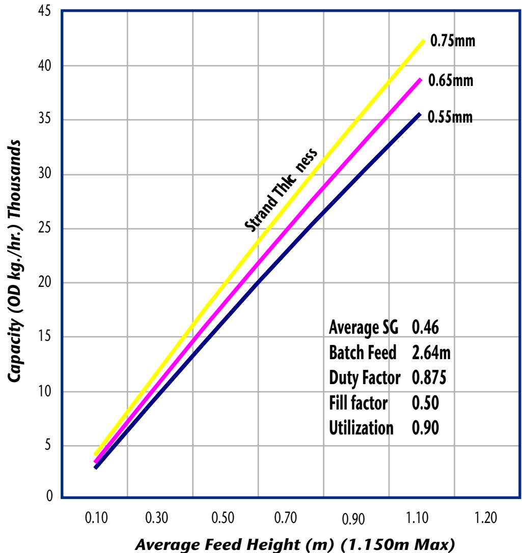
Carmanah 28/81 SmartRING Typical Capacity - Pine
